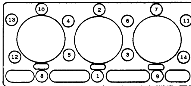
Figure 1-1. Cylinder Head Nut Tightening Sequence
